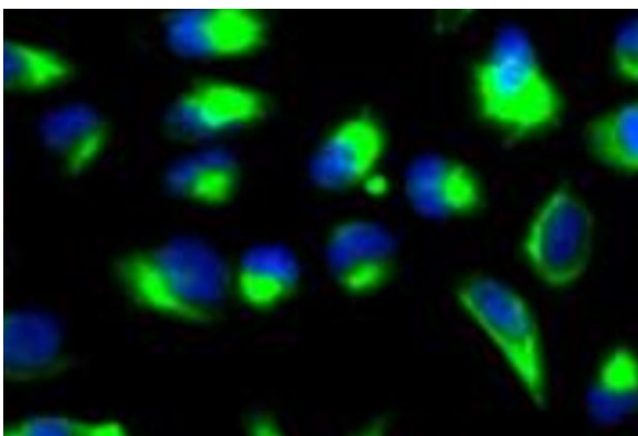
ARG46777 anti-CD86 antibody ICC/IF image
