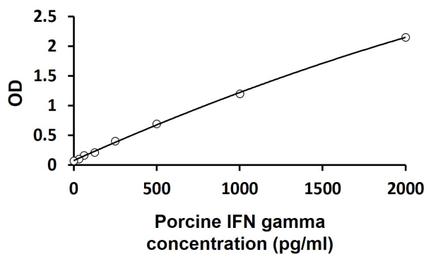
ARG80097 Porcine IFN gamma ELISA Kit standard curve image
