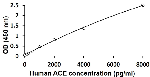
ARG80958 Human ACE ELISA Kit standard curve image
