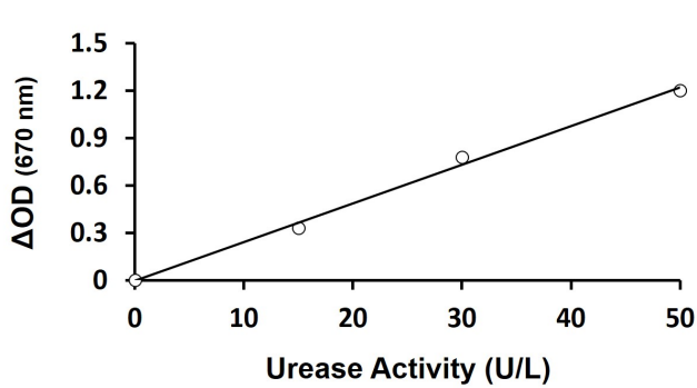
ARG82196 Urease Activity Assay Kit typical data demonstration image
