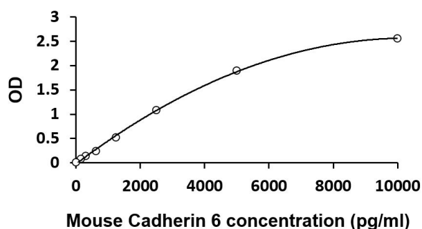
ARG82574 Mouse Cadherin 6 ELISA Kit standard curve image
