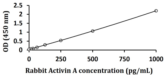
ARG83116 Rabbit Activin A ELISA Kit standard curve image
